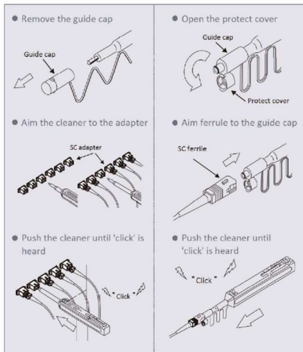
FC/SC/ST Operation Demonstration
